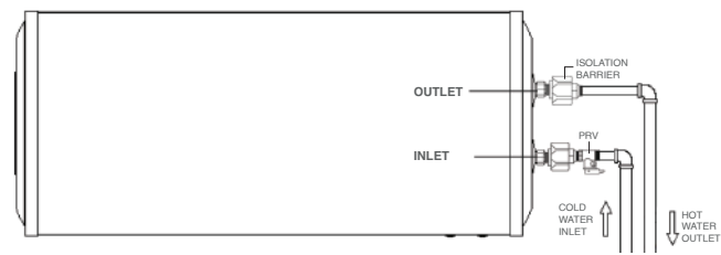
Pipe Connection
